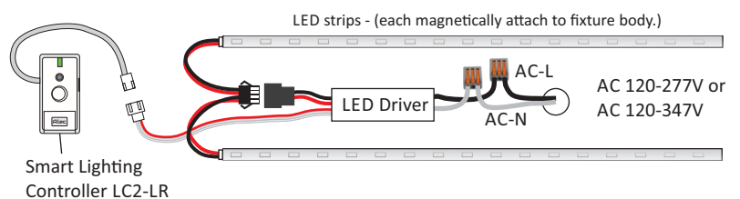
Figure 5: SLC components & Wiring Diagram
